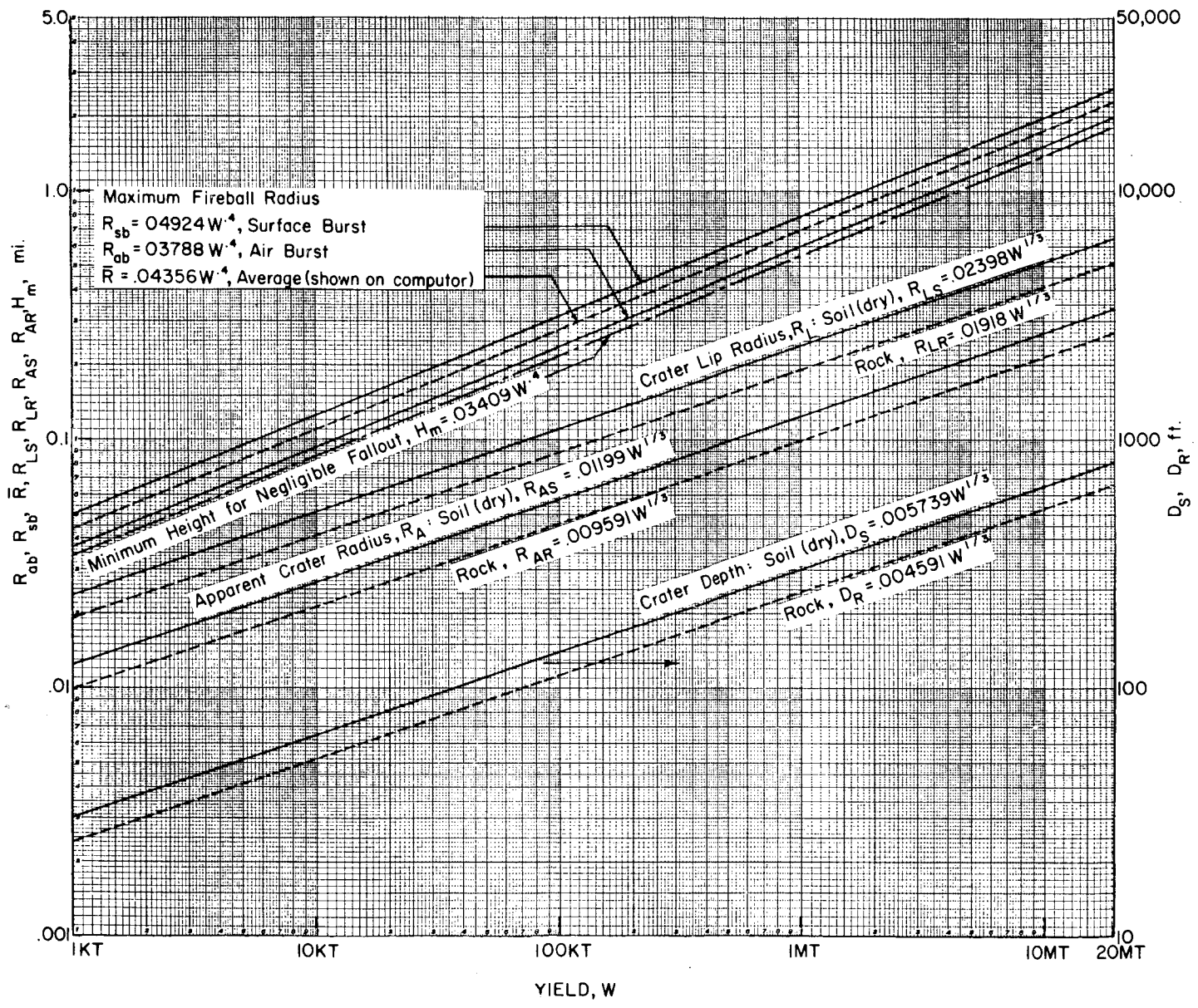
Fig. 2.19—Crater and fireball dimensions as a function of yield. Also shown are minimum heights of burst for negligible fallout vs. yield.
